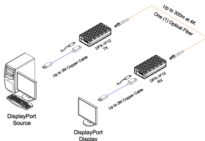
Figure 1 – Overall Connection of DPX-1F12-TR
